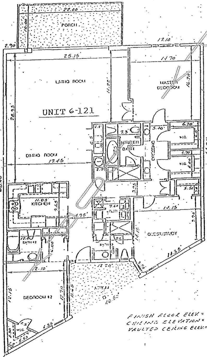
FLOOR PLAN SOUTHWINDS A UNIT 6-121 A CONDOMINIUM
