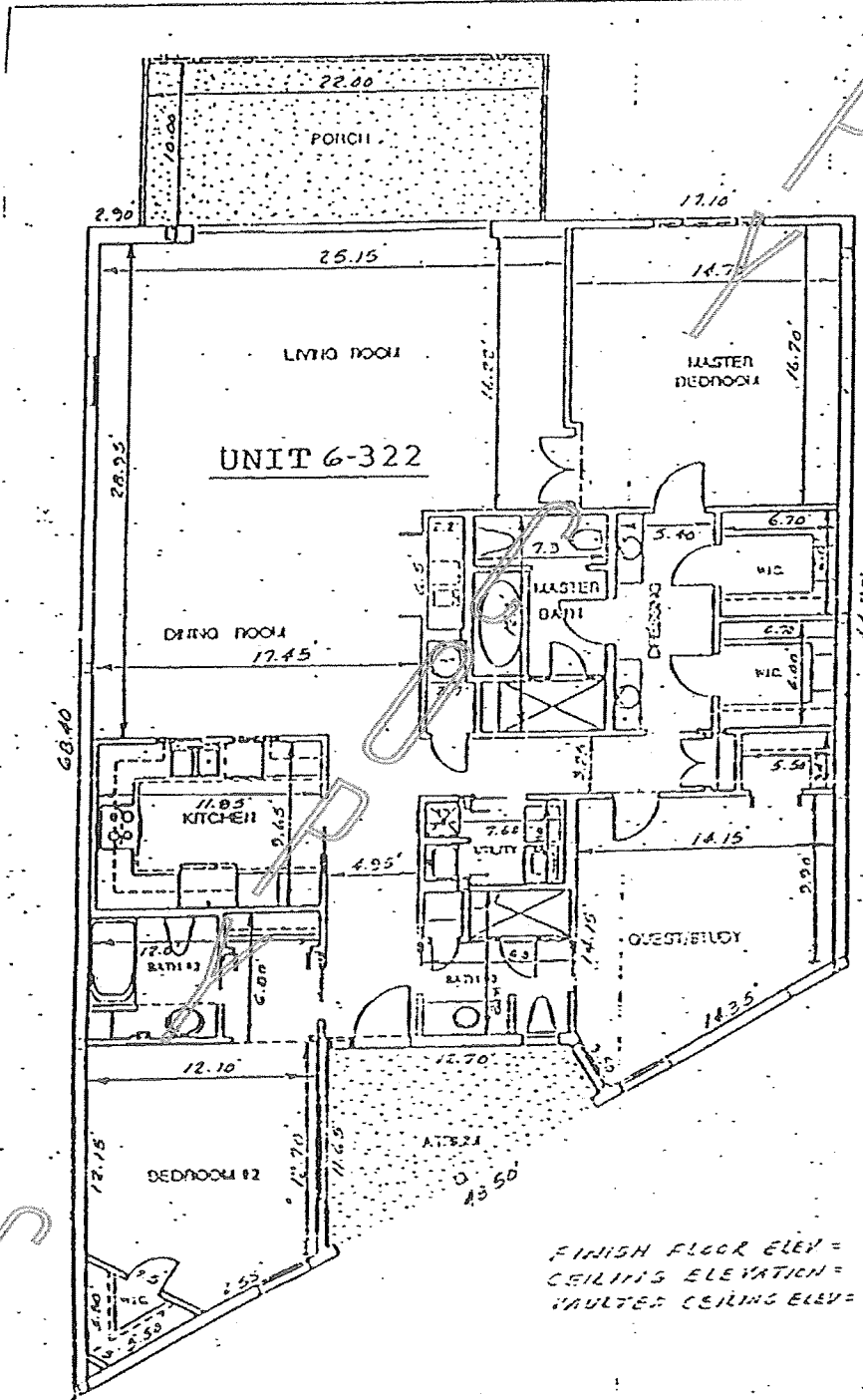
FLOOR PLAN SOUTHWINDS A UNIT 6-322 A CONDOMINIUM
